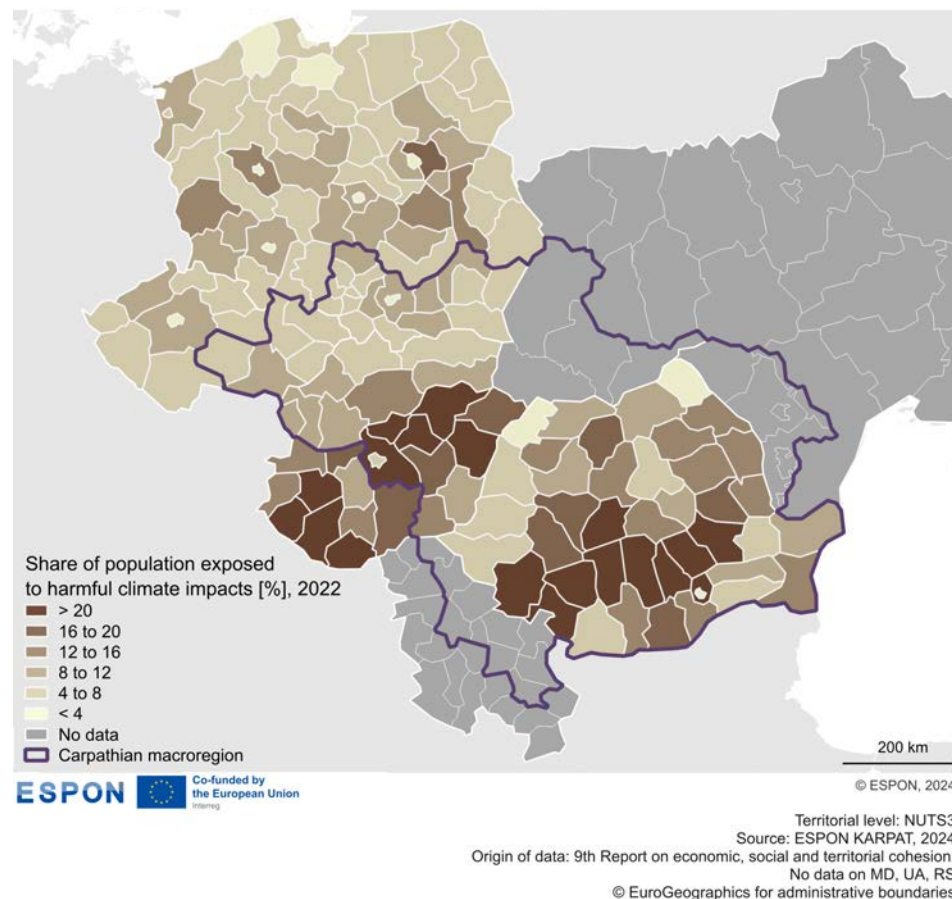
Map 16. Share of population exposed to harmful climate impacts, 2022
